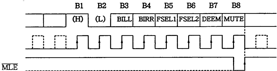
Fig. 17 Mode flag Timing 1
