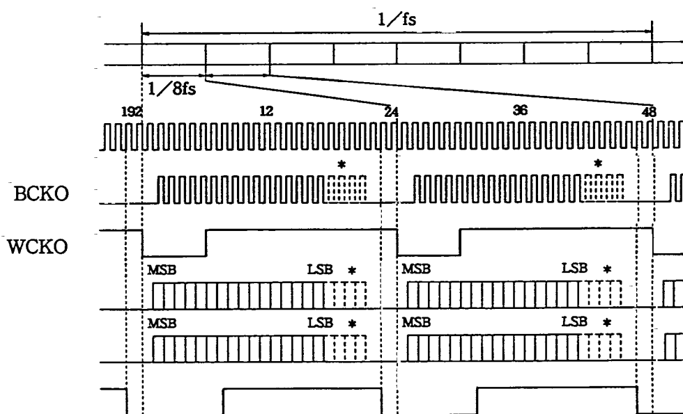
Fig. C Example 1 ( \overline{\text{CKSL}} = H, OMOD flag = L)
