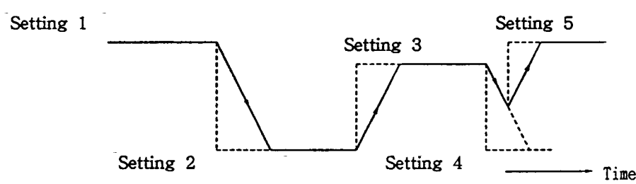
Fig. 16 Attenuation Level Transitions Setting
