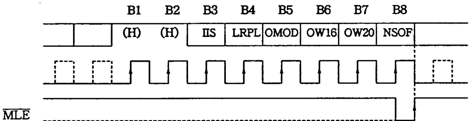
Fig. 18 Mode flag Timing 2
