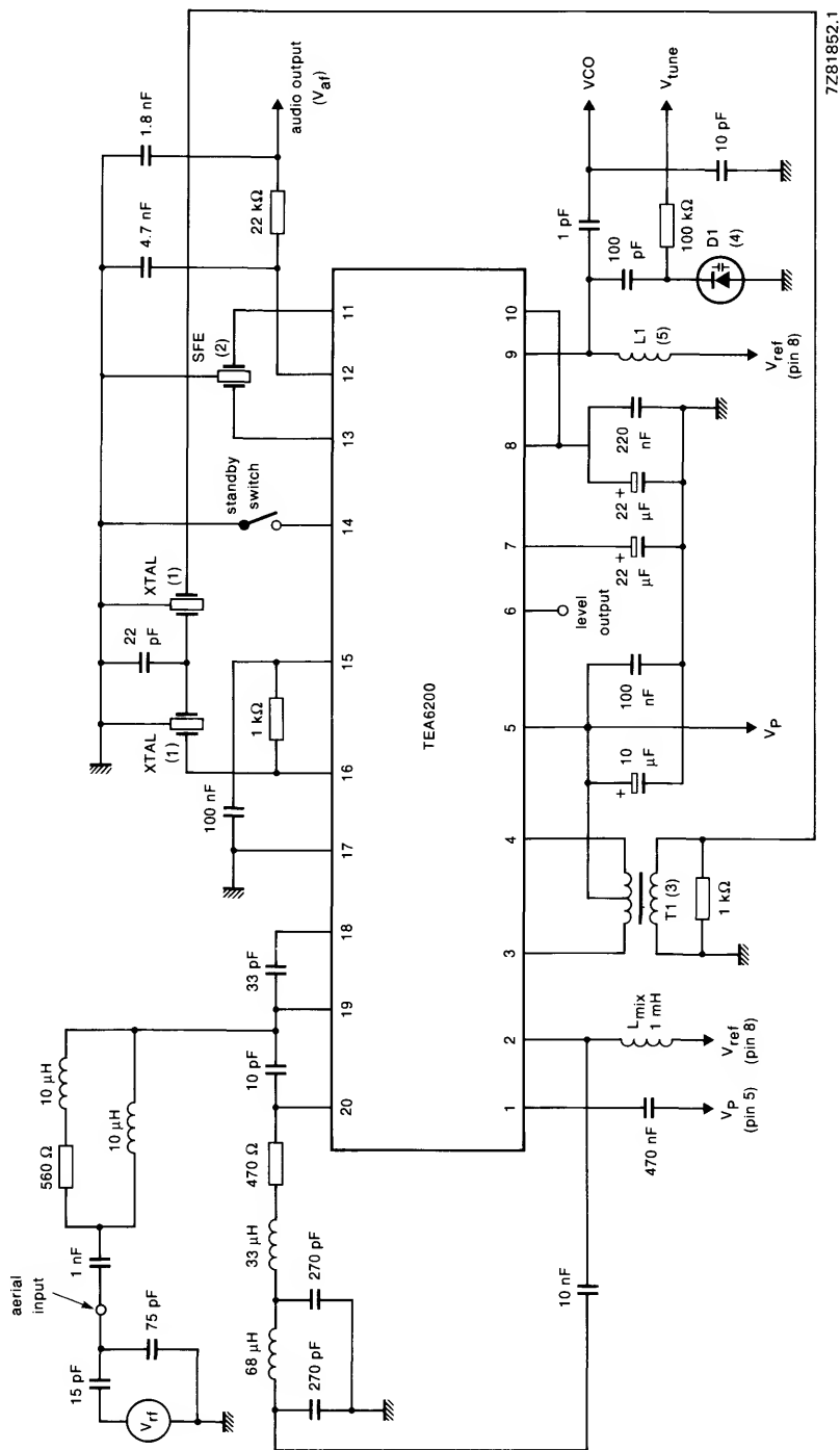
Fig. 8 Application diagram.
