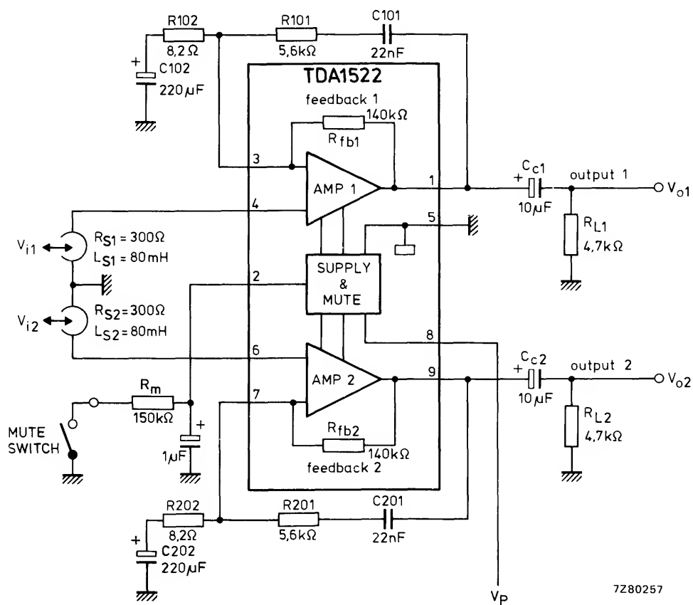
Fig. 9 Simple mute application.
