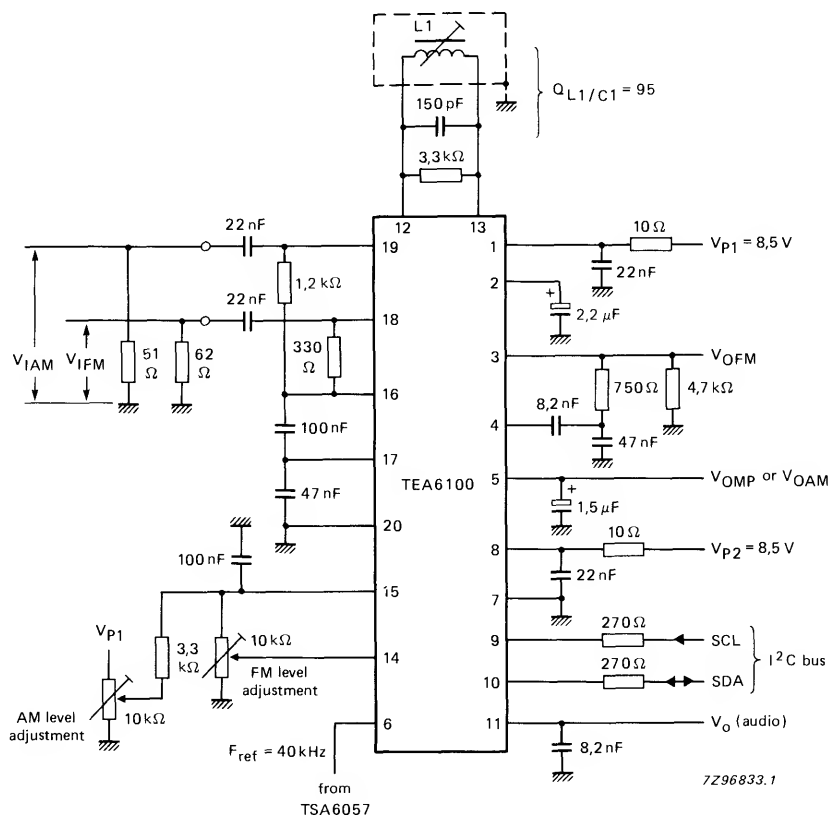
Fig. 13 Application diagram.
