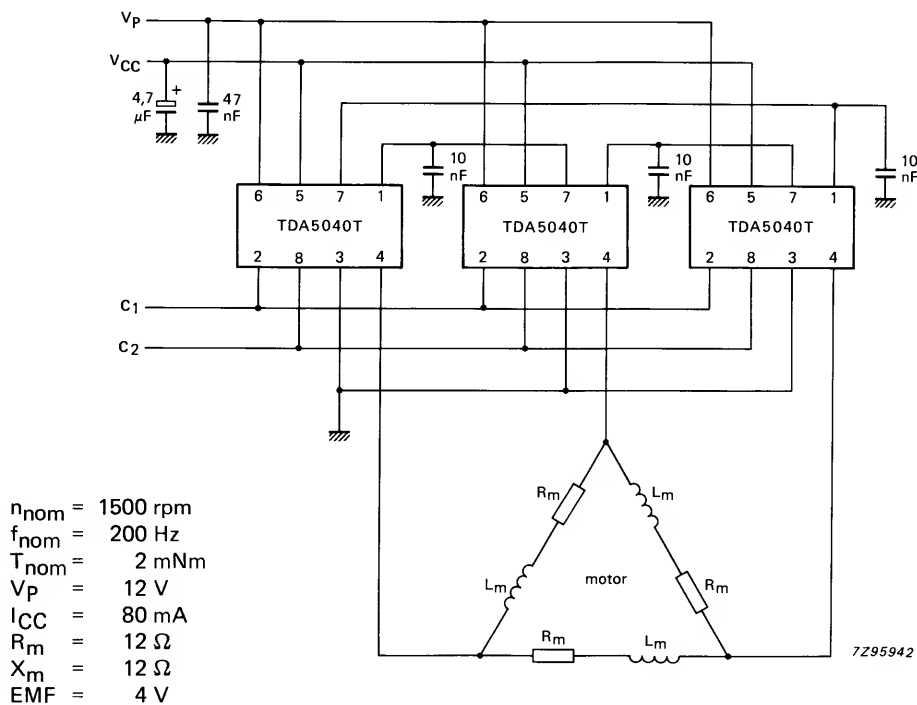
Fig. 5 Typical application circuit.
