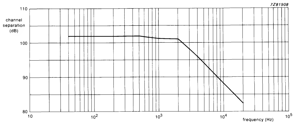
Fig. 12 Source selector separation (channel 2 and channel 1); gain = 0 dB; V_{i1} = 0 V; V_{i2} = 1 V, R_S = 0 \Omega ; R_L = 10 \text{ k}\Omega ; bass/treble = 0 dB; V_{CC} = 12 V.
