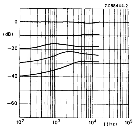
Fig. 9 Encoder frequency response for B-mode.
