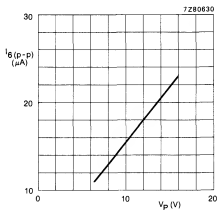
Fig. 5 Signal handling range at the input for I_{6(p-p)} ( \pm 75 kHz); V_{g.7} = V_P .
