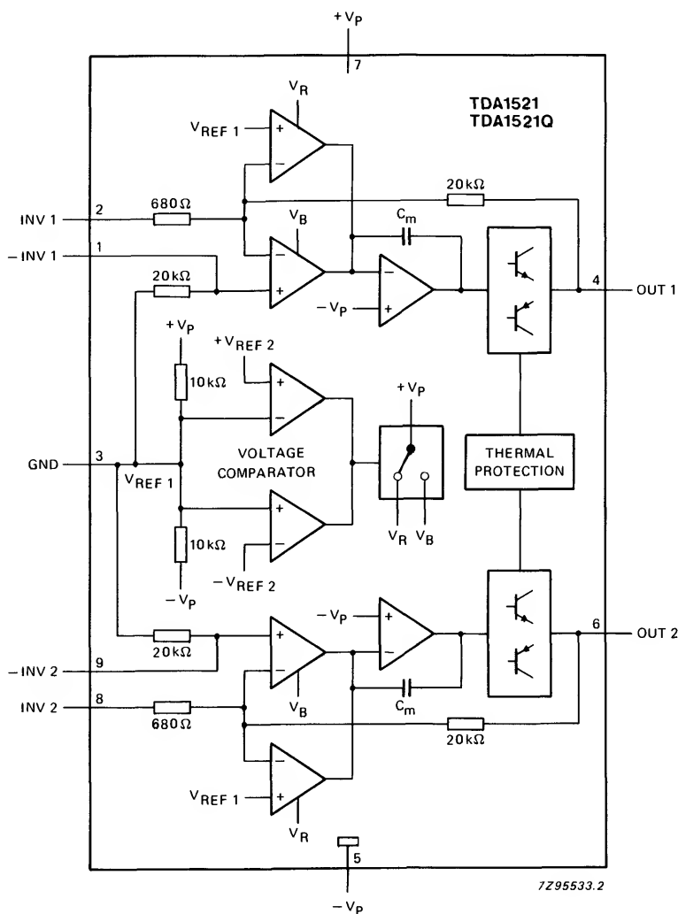
Fig. 1 Block diagram.
