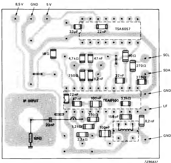
Fig. 14 Track side of printed circuit board.
