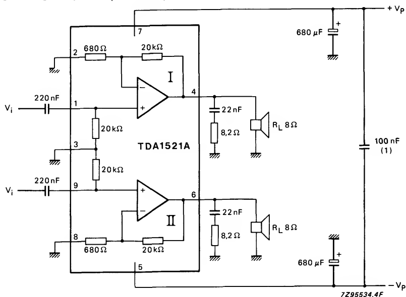
Fig. 11 Test and application circuit; symmetrical power supply.
