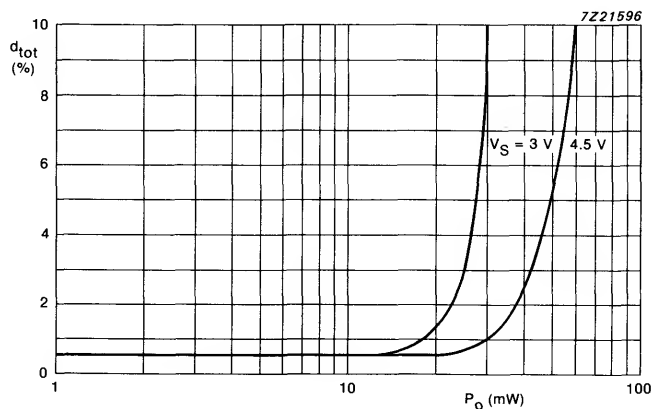
Fig. 5 Total distortion ( d_{\text{tot}} ) as a function of output power ( P_o ).
