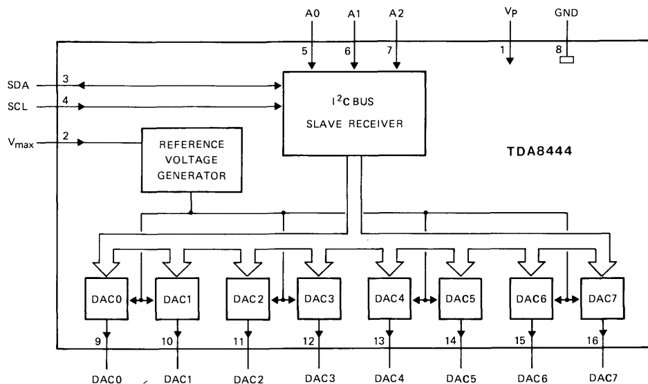
Fig. 1 Block diagram.
