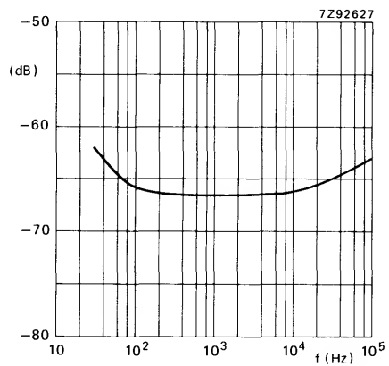
Fig. 15 Crosstalk from record input (pin 26) to line output as a function of frequency in playback mode; record input level is 50 mV; NR OFF; R_G = 10 k \Omega .
