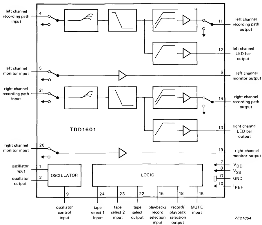
Fig. 1 Block diagram.
