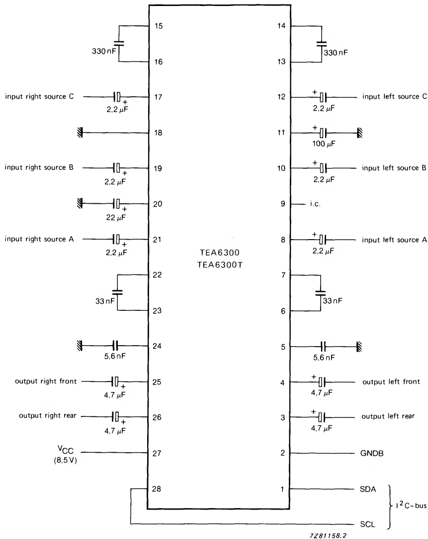
Fig. 10 Test and application circuit.
