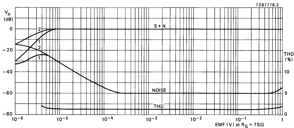
Fig. 4 Mono operation: AF output voltage ( V_o ) and total harmonic distortion (THD) as functions of input e.m.f. (EMF); R_{source} = 75 \Omega ; f_{rf} = 96 \text{ MHz} ; 0 dB = 90 mV. For S+N and noise curves (1) is with muting enabled and (2) is with muting disabled; signal \Delta f = \pm 22,5 \text{ kHz} and f_m = 1 \text{ kHz} . For THD curve, \Delta f = \pm 75 \text{ kHz} and f_m = 1 \text{ kHz} .
