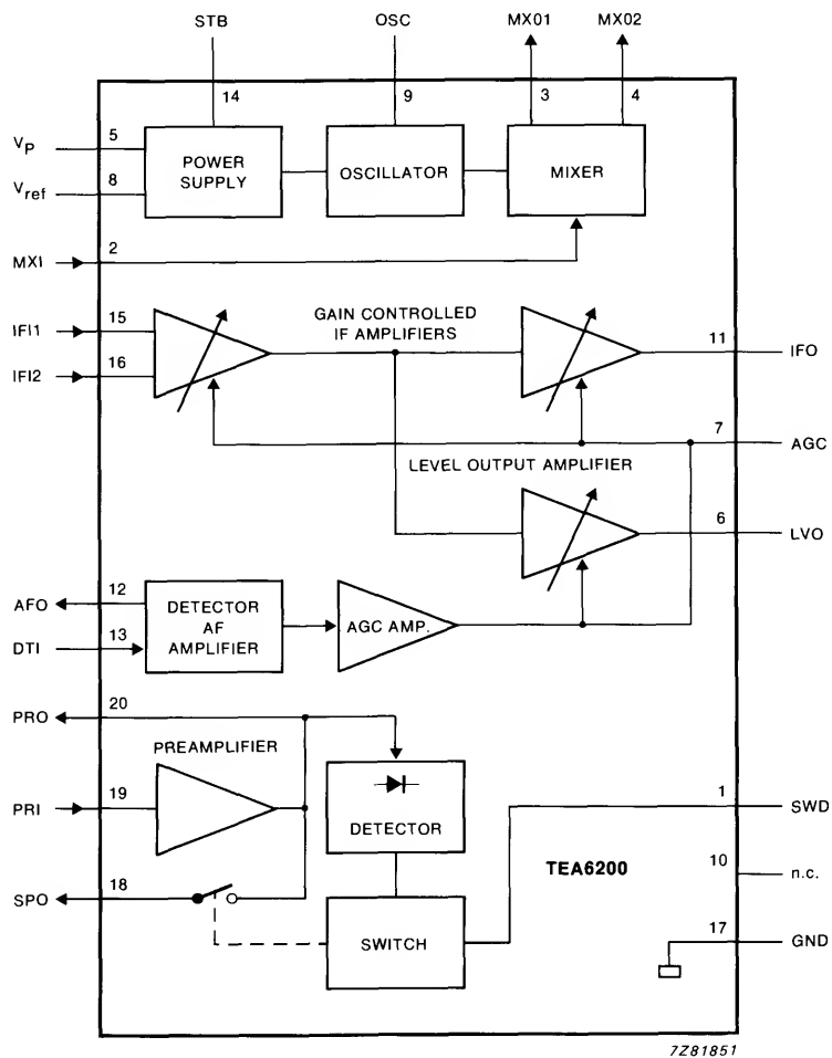
Fig. 1 Block diagram.
