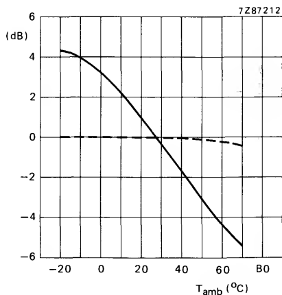
Fig. 7 Sensitivity ( V_i ), output voltage ( V_O ) as a function of temperature behaviour ( T_{amb} ). Measured at f_i = 10,7 MHz in test circuit Fig. 10.
