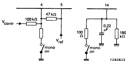
Fig. 3 (a) At pin 4; -V_{4.5} > 300 mV; (b) at pin 14.
