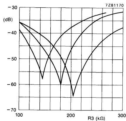
Fig. 8 Random samples of pilot cancelling: V_O (at 19 kHz) / V_O (at 1 kHz) in dB as a function of R_3 ; V_{i(p-p)} = 1 V; V_{pilot} = 32 mV (9%).
