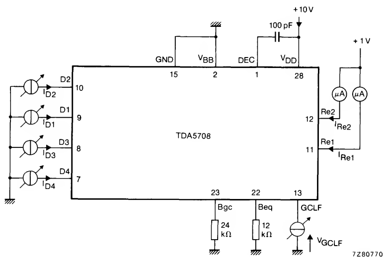
Fig. 9 Test circuit for output current I_{Re1} and I_{Re2} .
