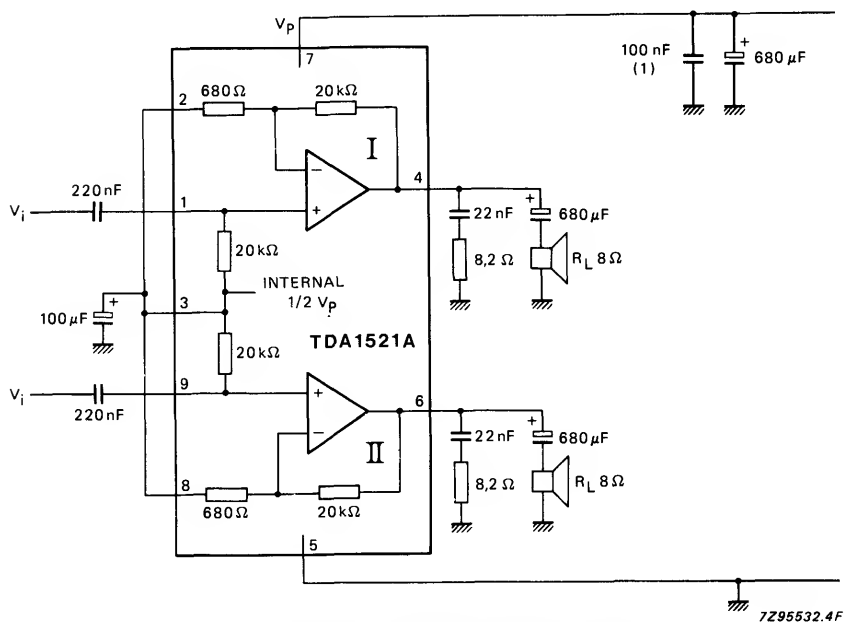
Fig. 12 Test and application circuit; asymmetrical power supply.
