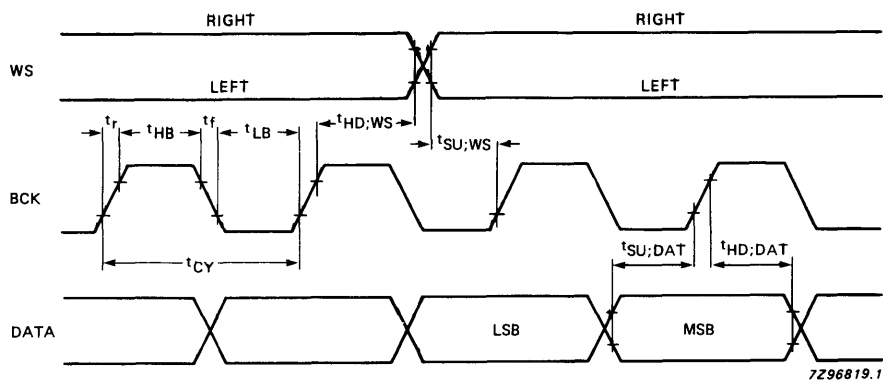
Fig. 3 Format of input signals; time multiplexed (I²S format).
