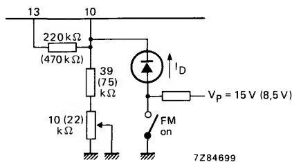
Fig. 4 The oscillator is switched-off when: I_D > 100 \mu\text{A} ( > 50 \mu\text{A} for V_p = 8.5 V) and I_D < 1 mA.
