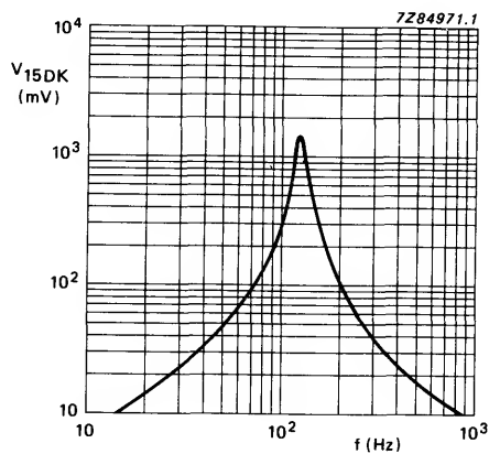
Fig. 3 DK signal voltage at pin 15 as a function of frequency: f_0 = 125 Hz; Q \approx 18 .
