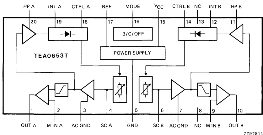
Fig. 1 Block diagram.
