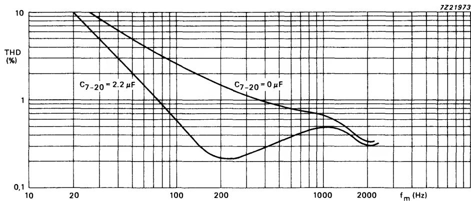
Fig. 5 Total harmonic distortion as a function of modulation frequency at V_i = 5 mV; m = 80\% ; measured in the circuit of Fig. 1 with C_{7-20}(\text{ext}) = 0 \mu F and 2.2 \mu F .
