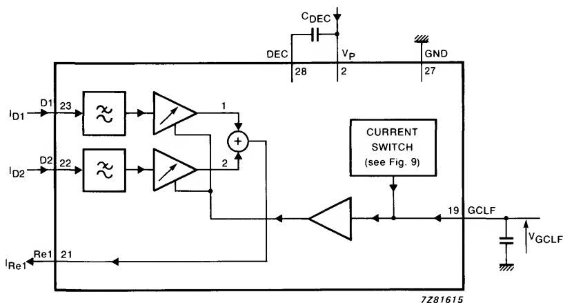
Fig. 7 Block diagram; (D1 + D2) input to Re1 output.
