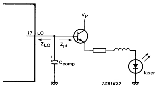
Fig. 18 Laser amplifier output circuitry.
