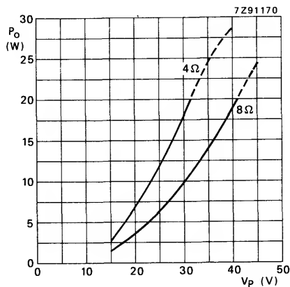
Fig.3 Output power ( P_O ) versus supply voltage ( V_P ); f = 1 kHz; d_{tot} = 0.5\% ; G_V = 30 dB.
