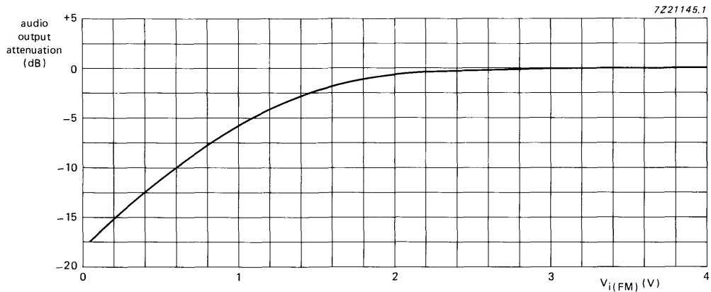
Fig. 11 Soft muting plotted against level output voltage; V_{i(FM)} = 1 mV and \Delta f = 22,5 kHz.
