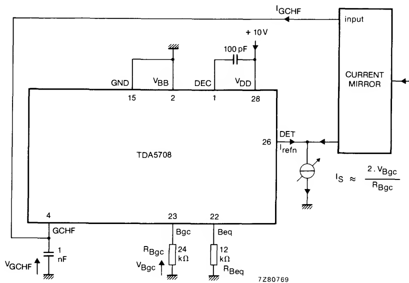
Fig. 8 Test circuit for negative reference current ( I_{refn} ).
