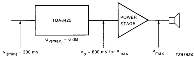
Fig. 24 Level diagram.
