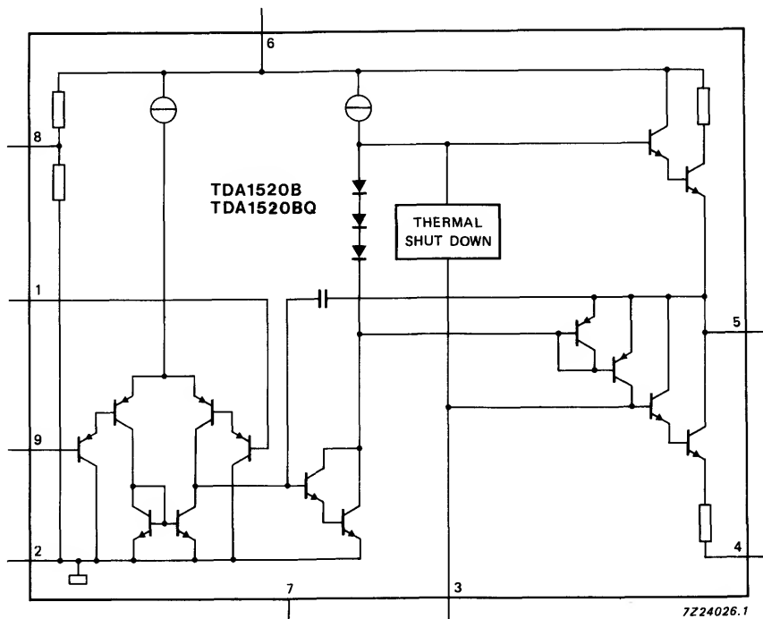
Fig. 1 Block diagram.
