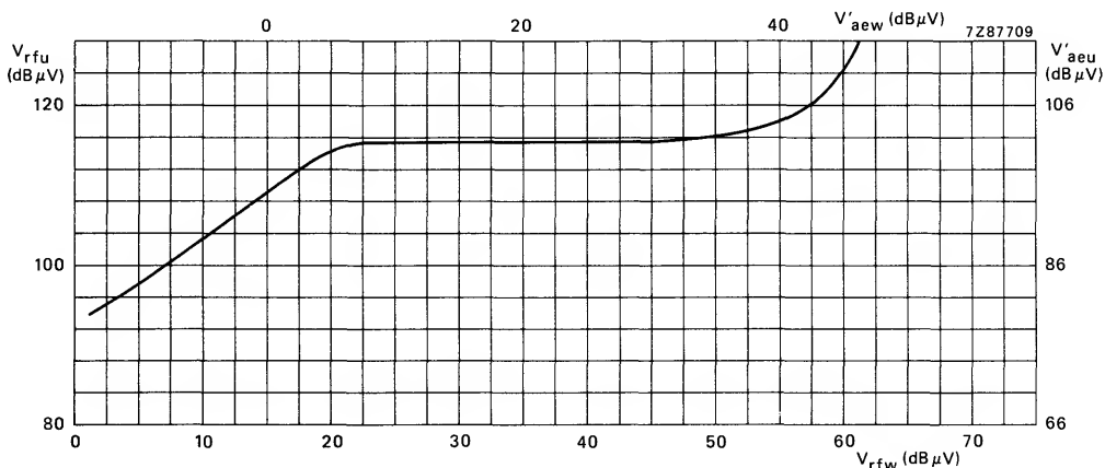
Fig. 10 Suppression of cross-modulation as a function of input signal, measured in the circuit of Fig. 8 with the input circuit as shown in Fig. 11. Curve is for Wanted V_{O(AF)}/\text{Unwanted } V_{O(AF)} = 20 \text{ dB} ; V_{rfw} , V_{rfu} are signals at the aerial input, V'_{aew} , V'_{aeu} are signals at the unloaded output of the aerial. Wanted signal ( V'_{aew} , V_{rfw} ): f_i = 1 \text{ MHz} ; f_m = 400 \text{ Hz} ; m = 30\% . Unwanted signal ( V'_{aeu} , V_{rfu} ): f_i = 900 \text{ kHz} ; f_m = 400 \text{ Hz} ; m = 30\% . Effective selectivity of input tuned circuit = 21 dB.
