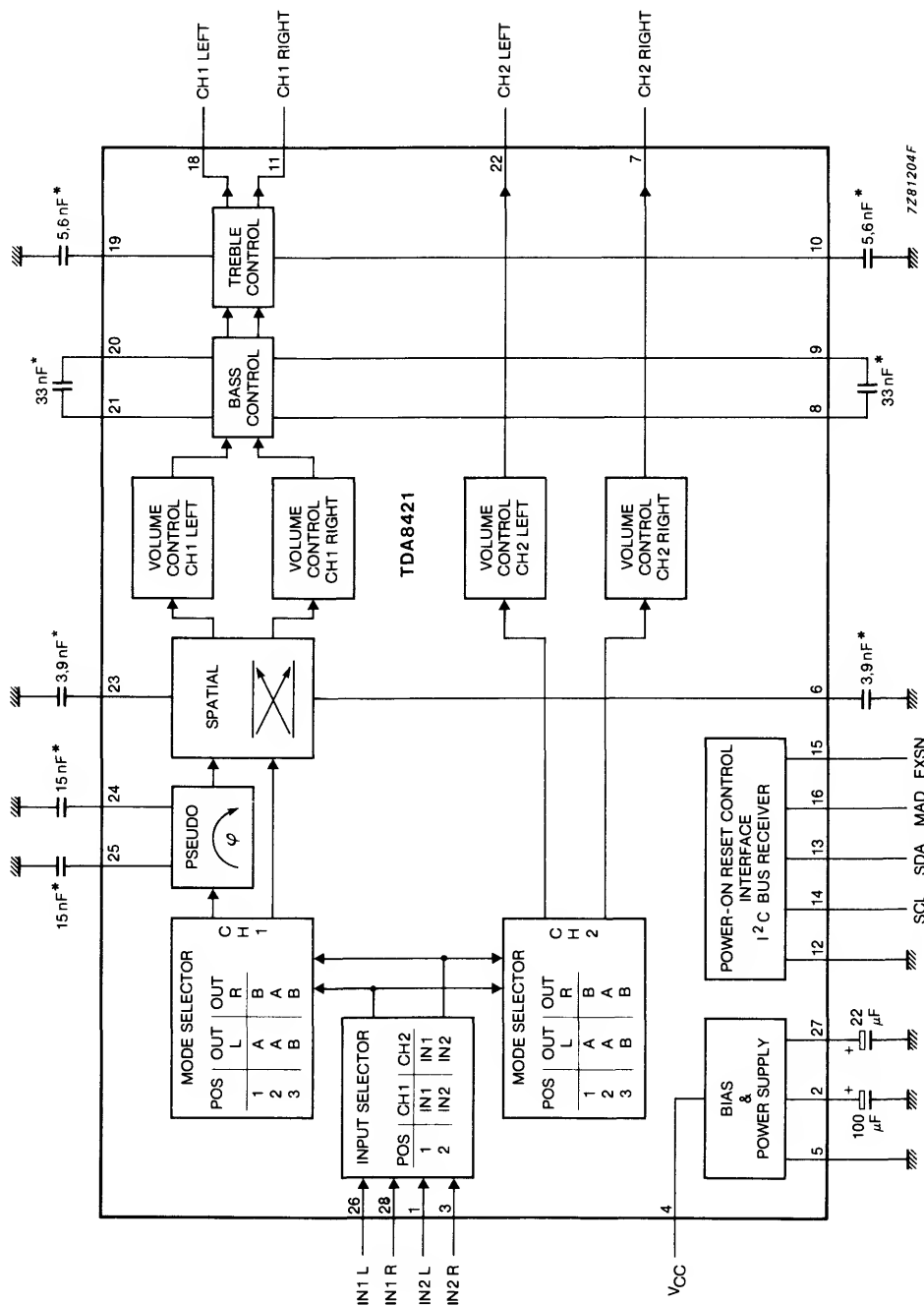
Fig. 1 Block diagram.
