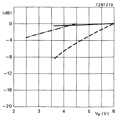
Fig. 8 Sensitivity ( V_i ) and output voltage ( V_O ) as a function of supply voltage ( V_P ). Measured at f_i = 10,7 MHz in test circuit Fig. 10.
