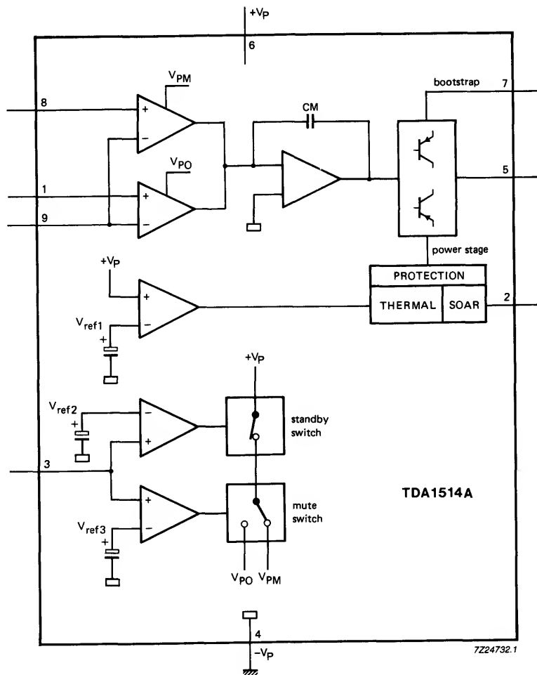
Fig.1 Block diagram.
