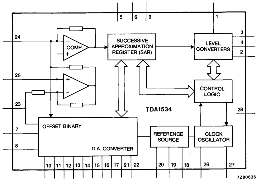
Fig. 1 Block diagram.
