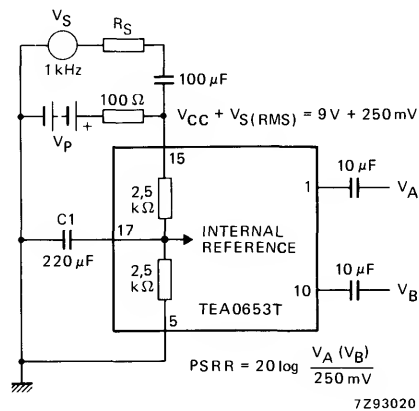
Fig. 3 Test circuit for PSRR for TEA0653T.
