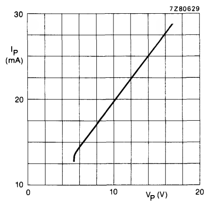
Fig. 6 Supply current consumption at I_P ; V_{g.7} = V_P .
