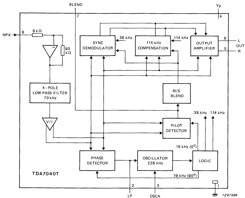
Fig. 1 Block diagram.
